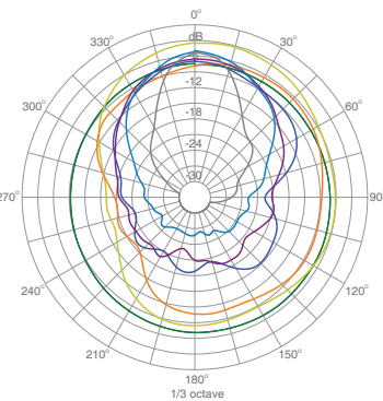
Directivity plot 101-14050 Hz 101 Hz 359 Hz 507 Hz 1000 Hz 2000 Hz 7551 Hz 14050 Hz
